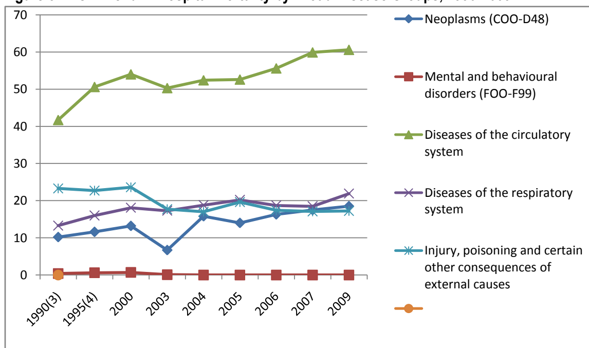
Figure 3 : NCD Trend in Hospital Mortality by Broad Disease Groups, 1990-2009
